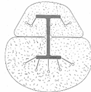
IPE 100 post covered with impact attenuator
