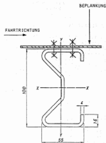
Fig. 2: Sigma guardrail post cross section
