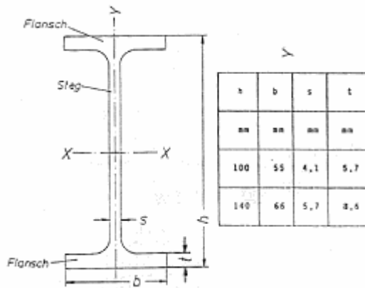
Fig. 1: IPE-100 guardrail post cross section
