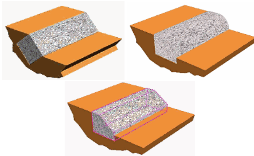
Fig. 10: making edges of sidewalks less aggressive to a fallen two-wheeler
